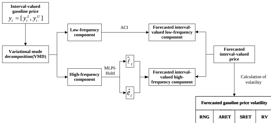
Figure 1 The framework of IHDE approach
