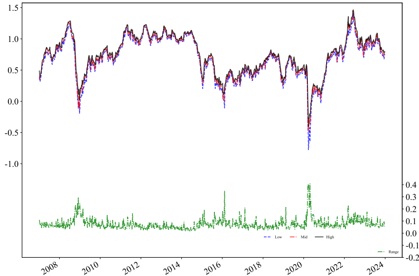
Figure 2 The weekly interval-valued gasoline price from Jan. 1, 2007, to Dec. 31, 2023
