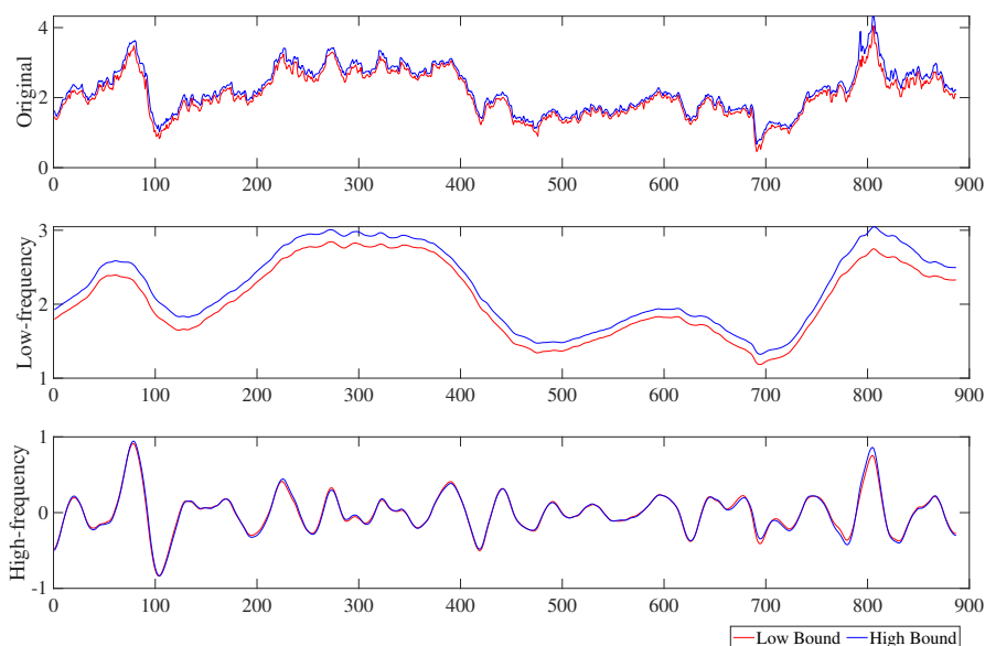
Figure 3 The MVMD results of weekly interval-valued gasoline price from Jan. 1, 2007, to Dec. 31, 2023
